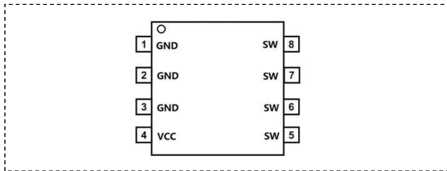
IW7707F (8 Lead SOIC-8 Package)
